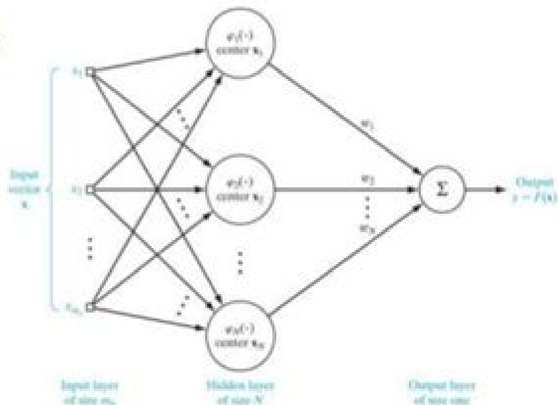
Figure 5.3 Structure of an RBF network , based on interpolation theory.
