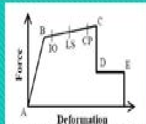
Figure 1: Force-Deformation for Pushover Hinge
