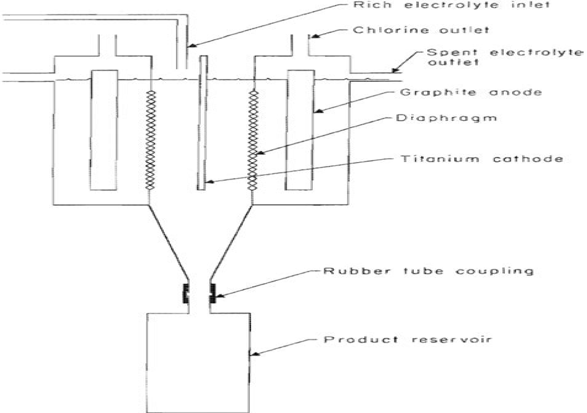
FIGURE 3. - Copper chloride electrolytic cell.
