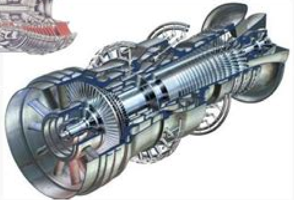
High Efficiency Power Generation Gas Turbine Engine with Sequential Combustion
