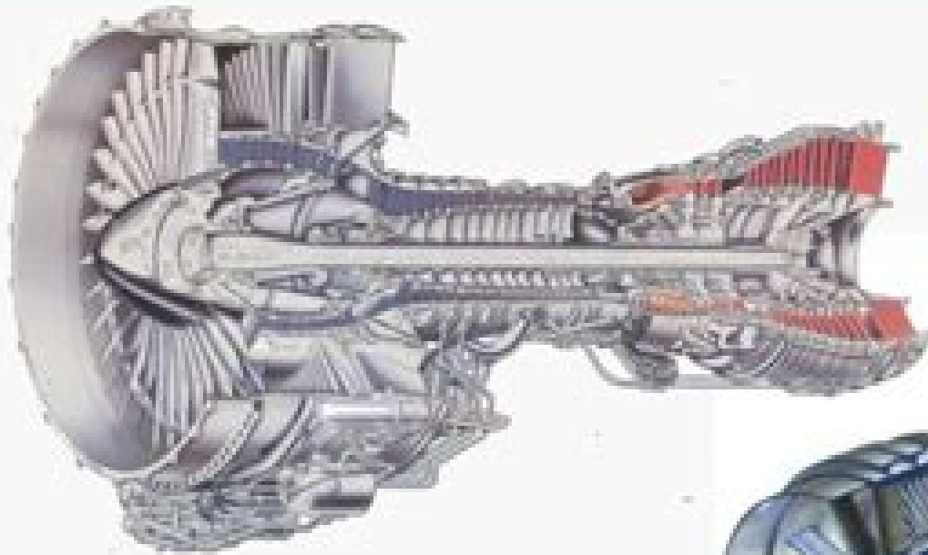
Twin-Spool Aircraft Gas Turbine Engine
