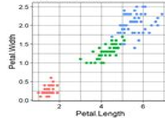
theme_linedraw()
