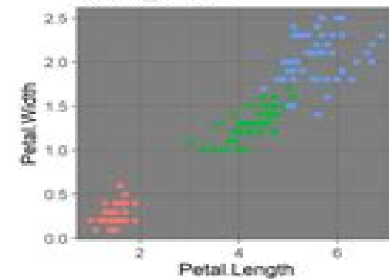
theme_dark()
