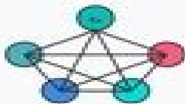
Complete Graph
