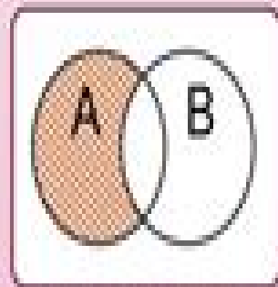
Set Difference A - B
