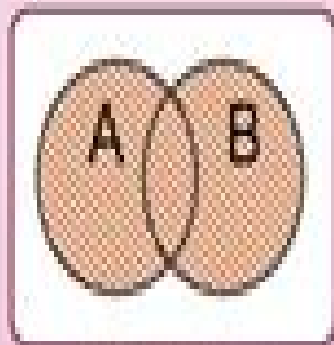
Set Union A \cup B
