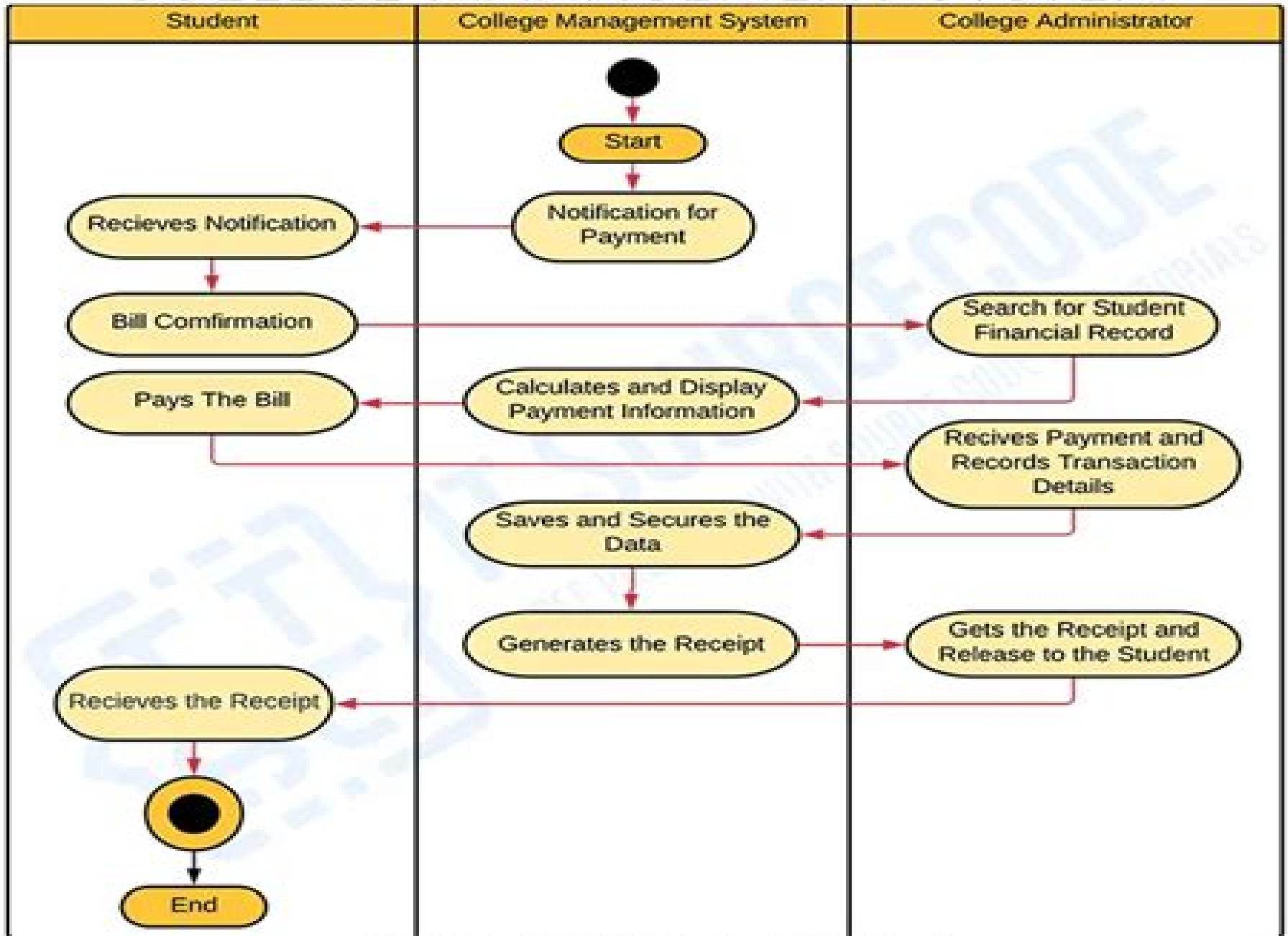
ACTIVITY DIAGRAM
