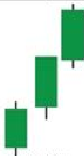
3 Soldier
