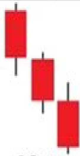
3 Crows
