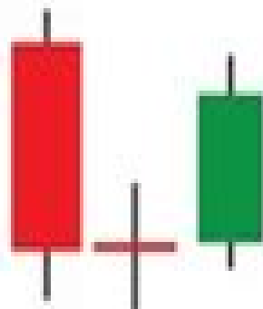
Morning Star
