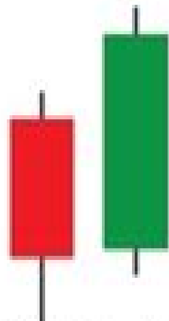
Bullish Engulfing
