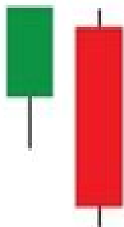
Bearish Engulfing
