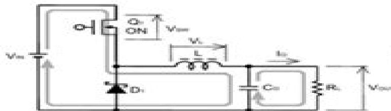
Fig. 1: Basic Buck Converter Circuit Switching Element ON
