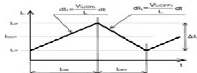
Fig. 3: Inductor Current Waveform
