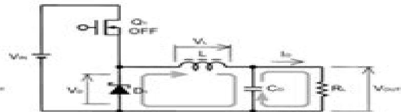
Fig. 2: Basic Buck Converter Circuit Switching Element OFF
