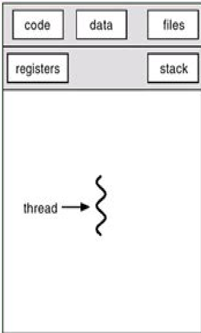
single-threaded
