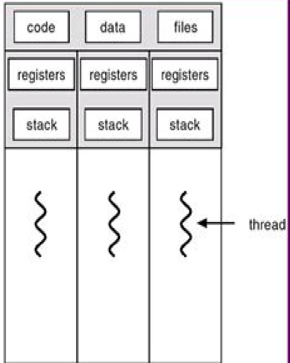
multithreaded
