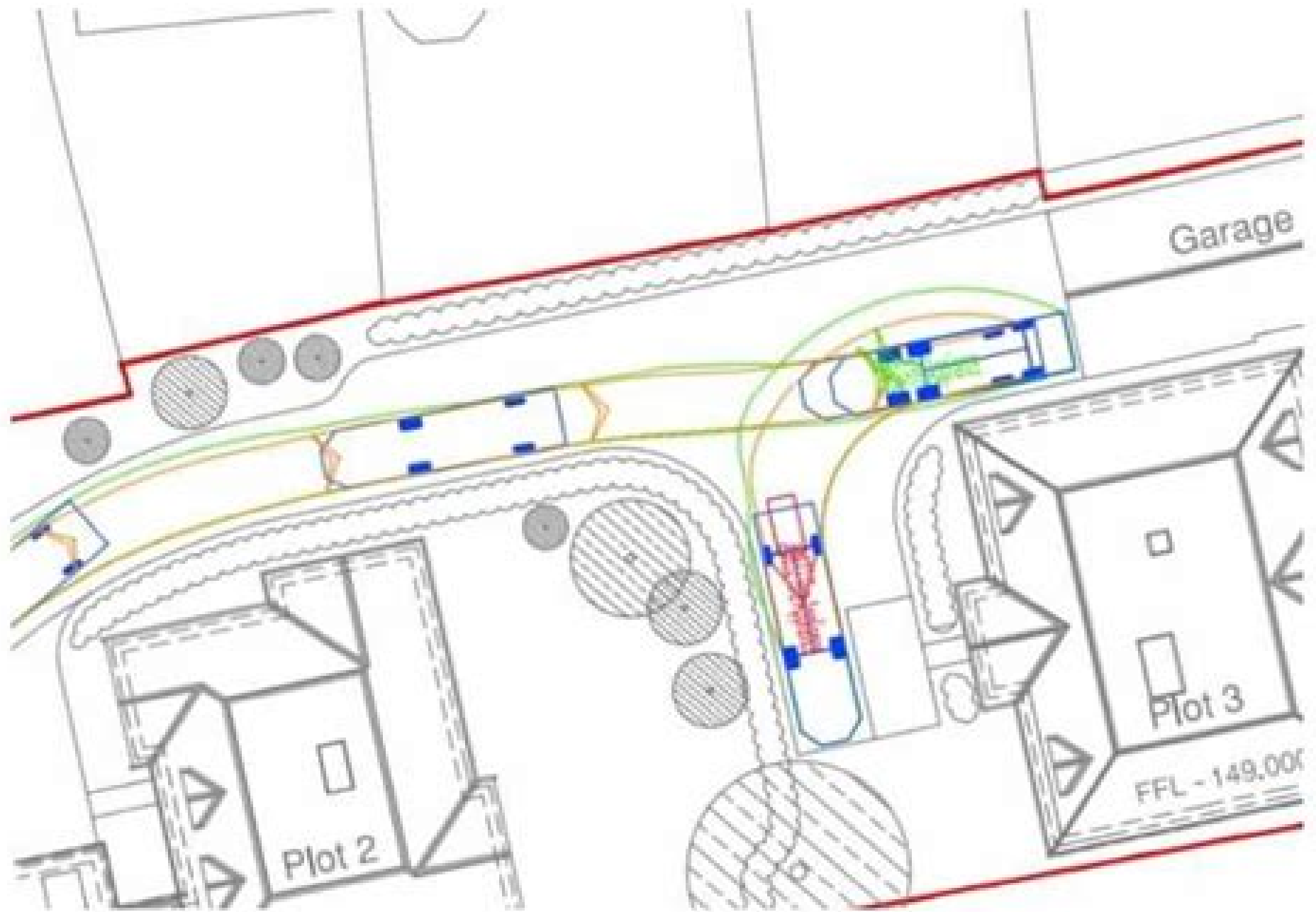
Swept Path Analysis example, Image provided by Lapworth Architects
