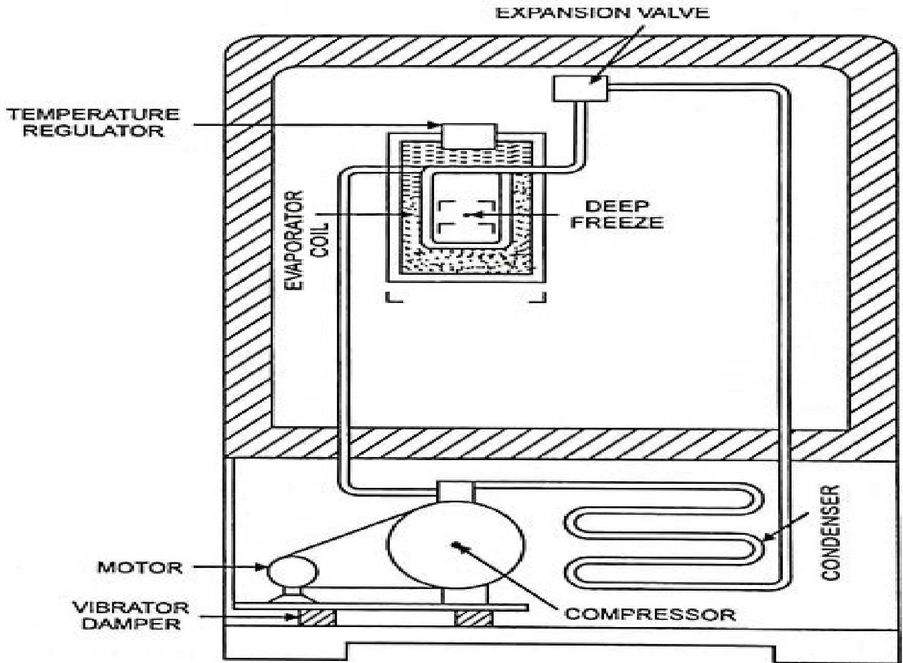
Fig. 9.6. Domestic Refrigerator
