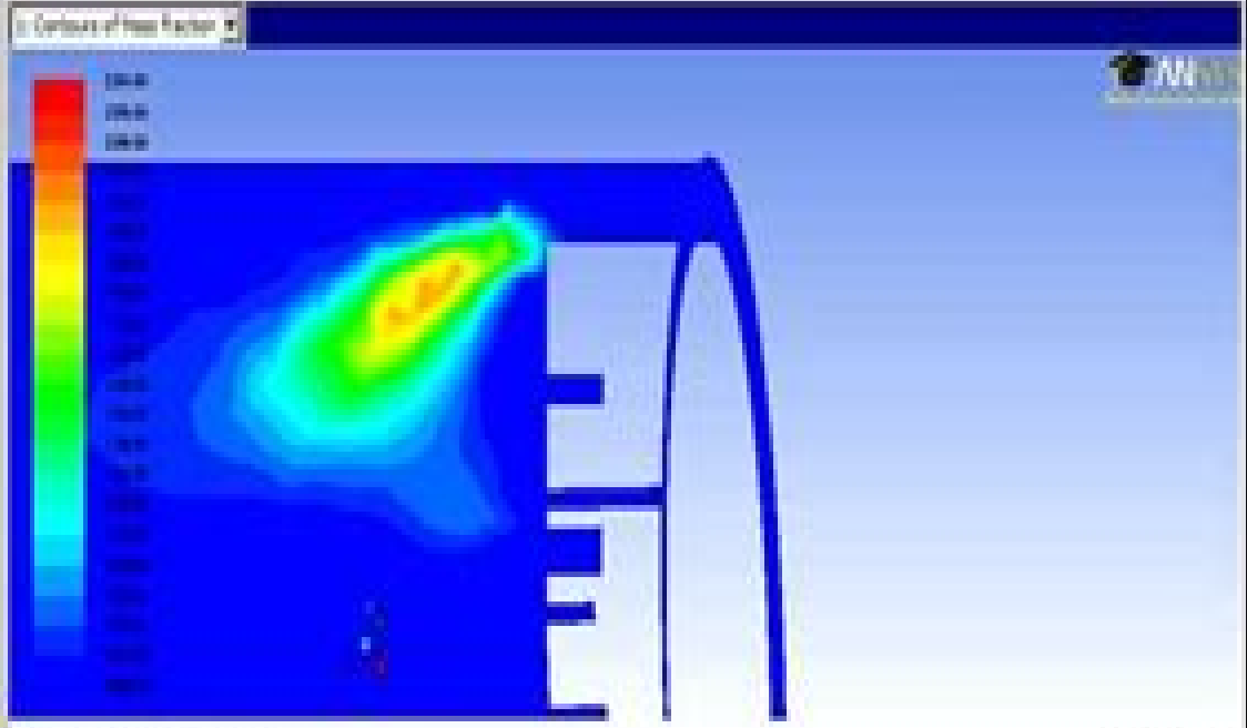
Contour of Mass Fraction of air
