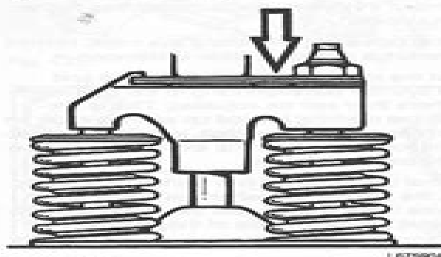
Fig. 139 Valve yoke
