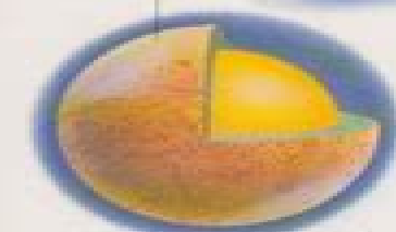
STRUCTURE OF PLUTO
