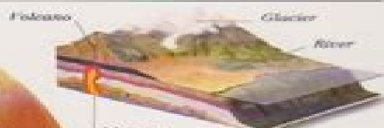
THE ROCK CYCLE
