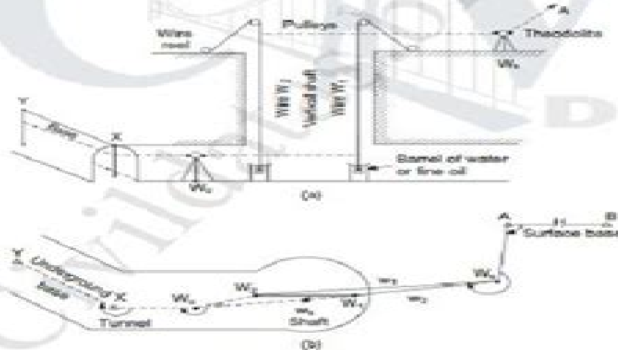
Fig. 10.34 (a) Section, and (b) plan
