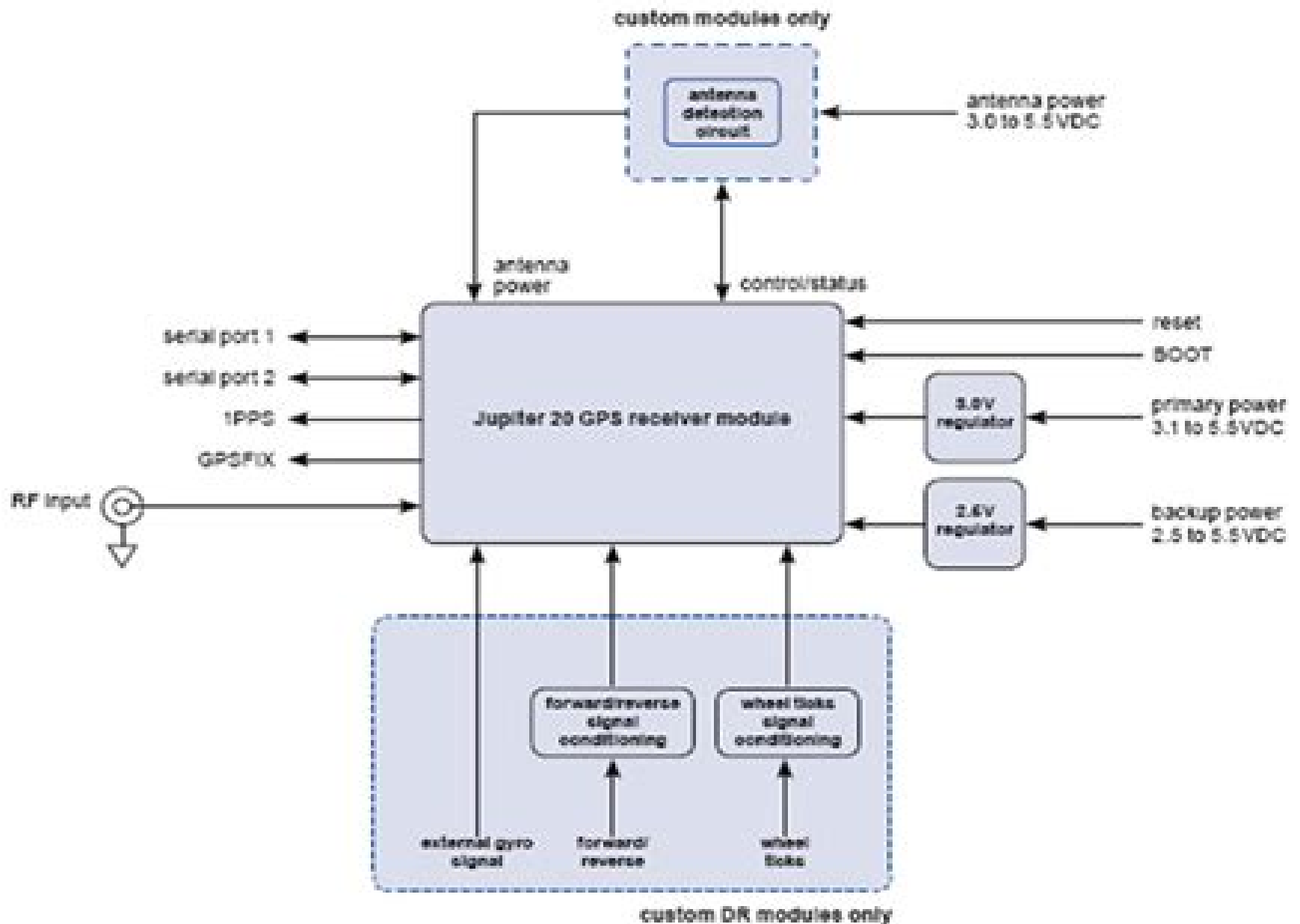
Jupiter 21 block diagram
