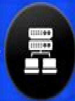
Object-Oriented Database
