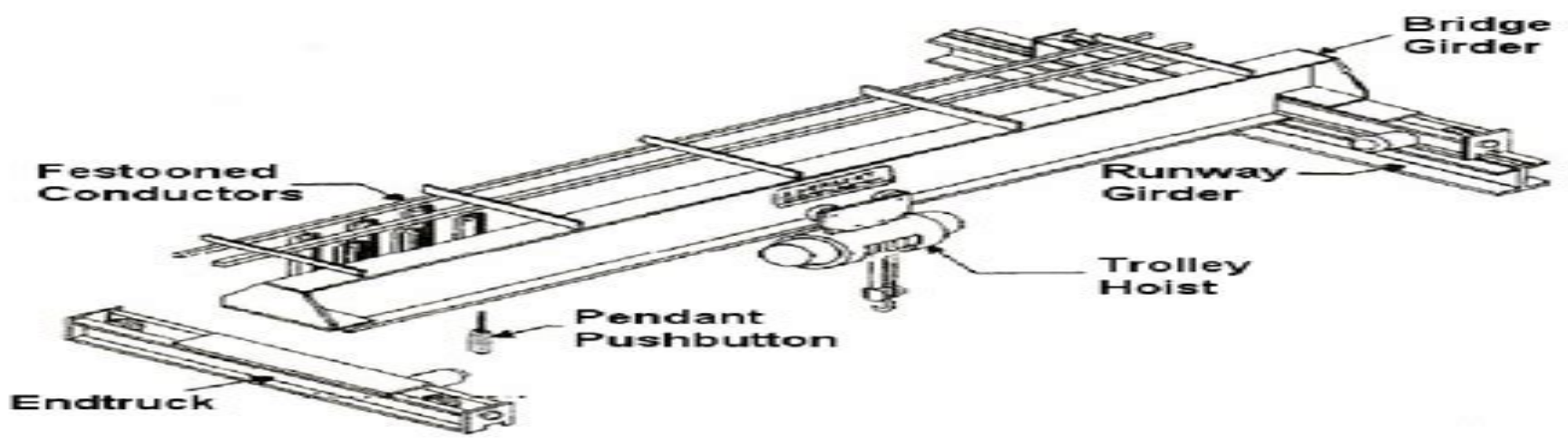
Figure 1. Single-beam overhead crane
