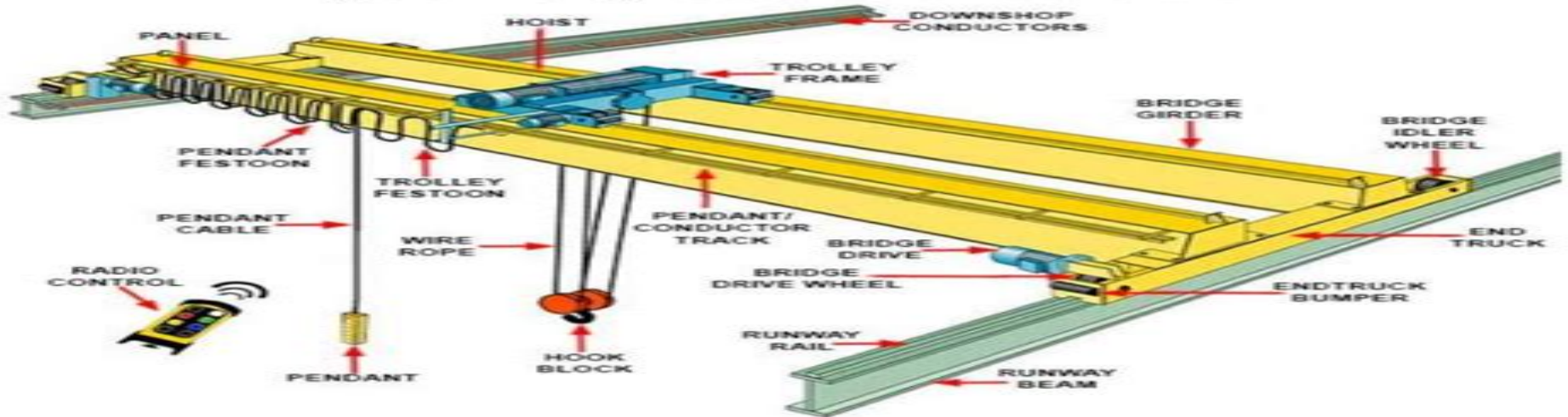
Figure 2. Double-beam overhead crane
