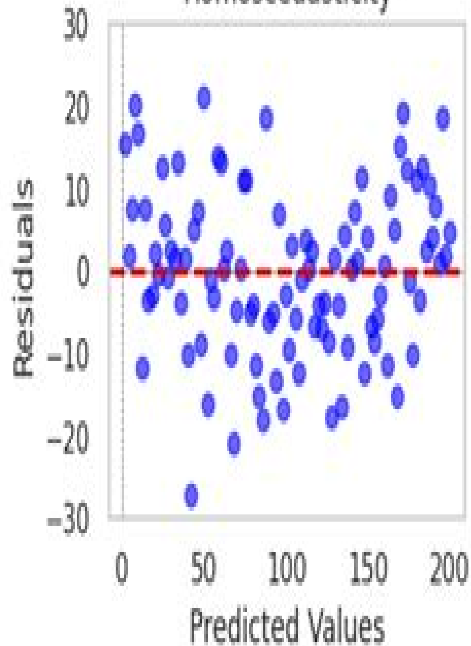
Homoscedasticity
