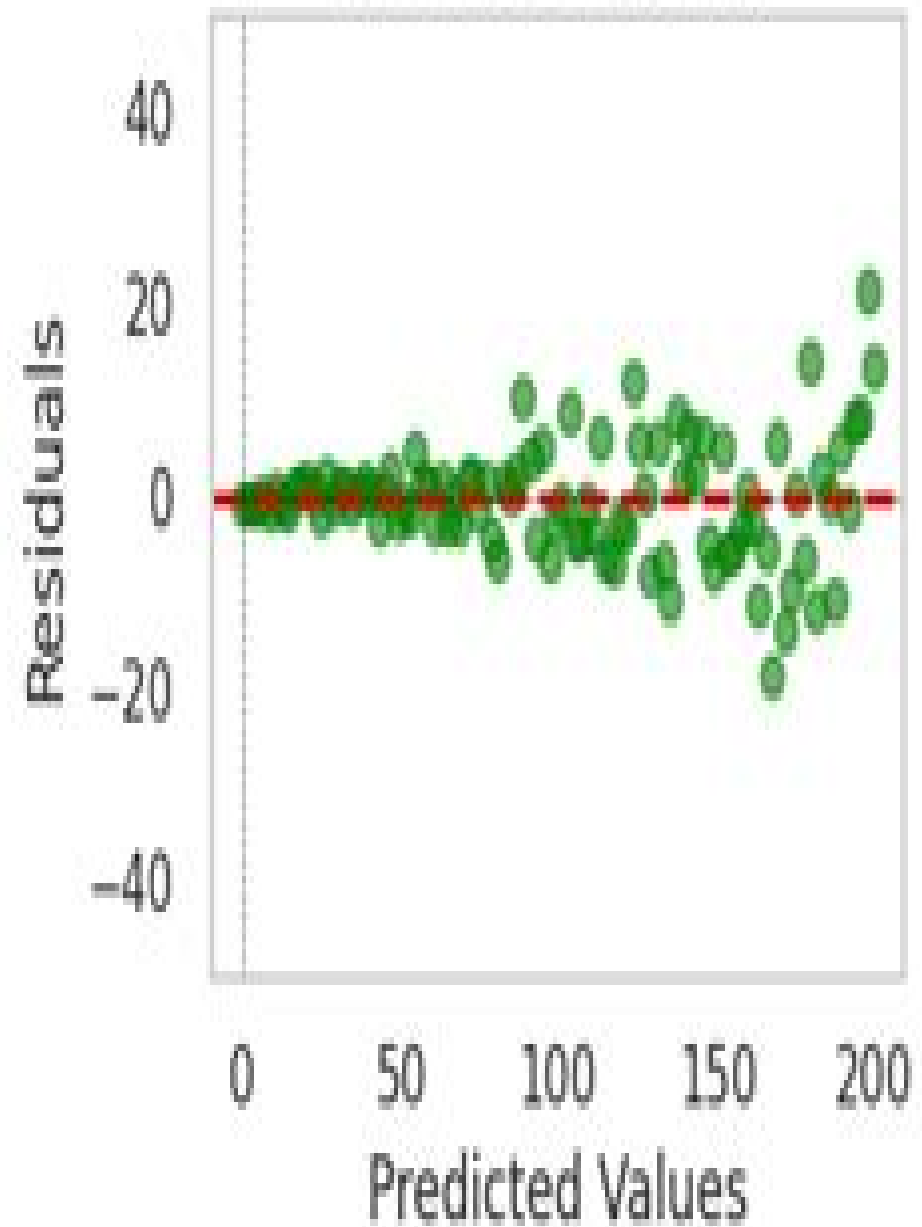
Heteroscedasticity
