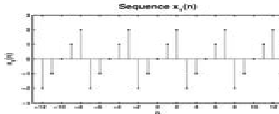
Figure 2.3.3: Problem P2.3.1 sequence plot
