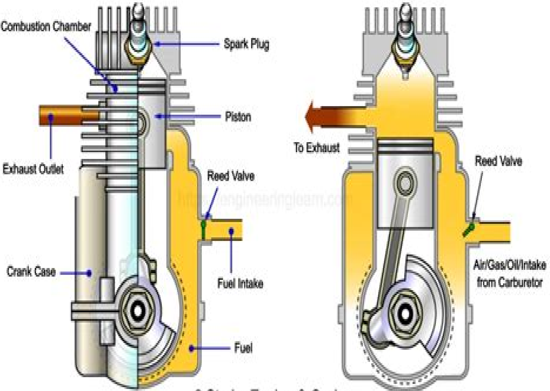
2 Stroke Engine & Cycle
