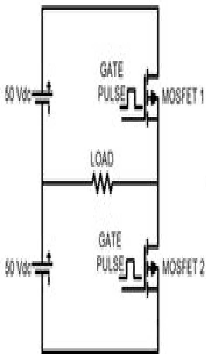
Half-Bridge Inverter
