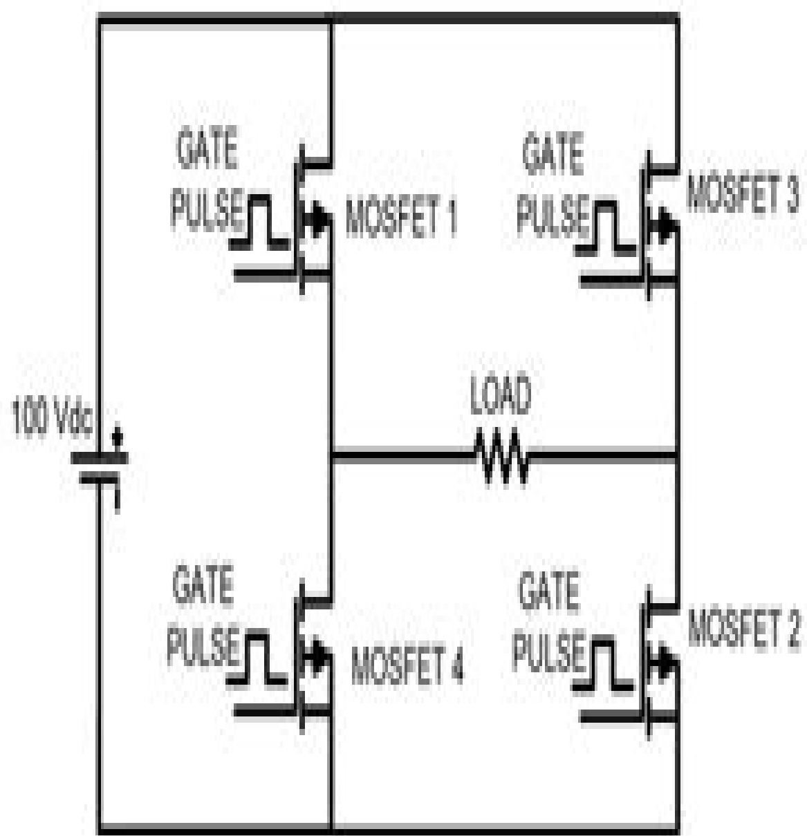
Full-Bridge Inverter
