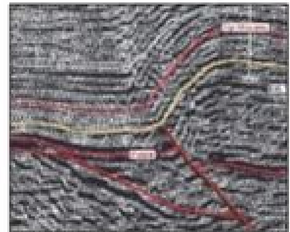
Seismic reflection
