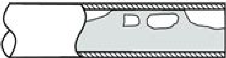
Intermittent flow
