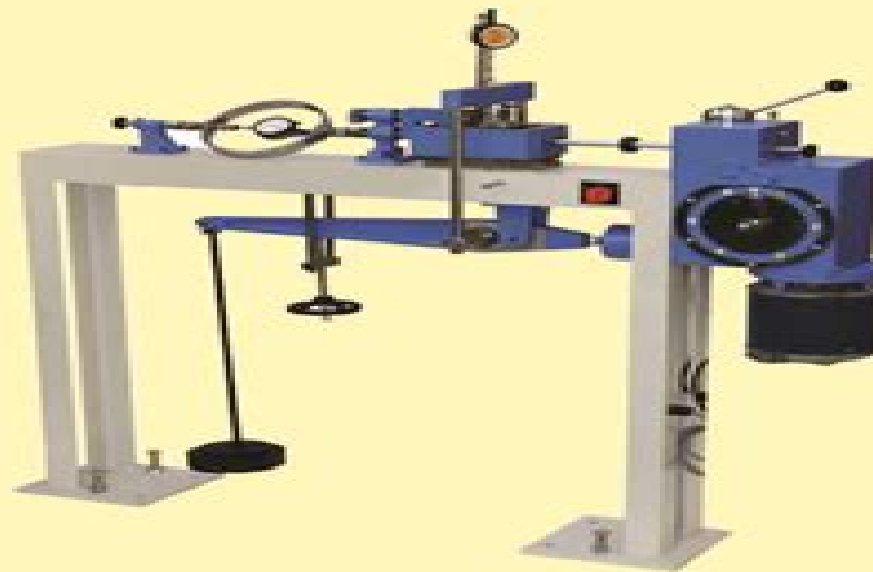
Direct Shear Test Apparatus
