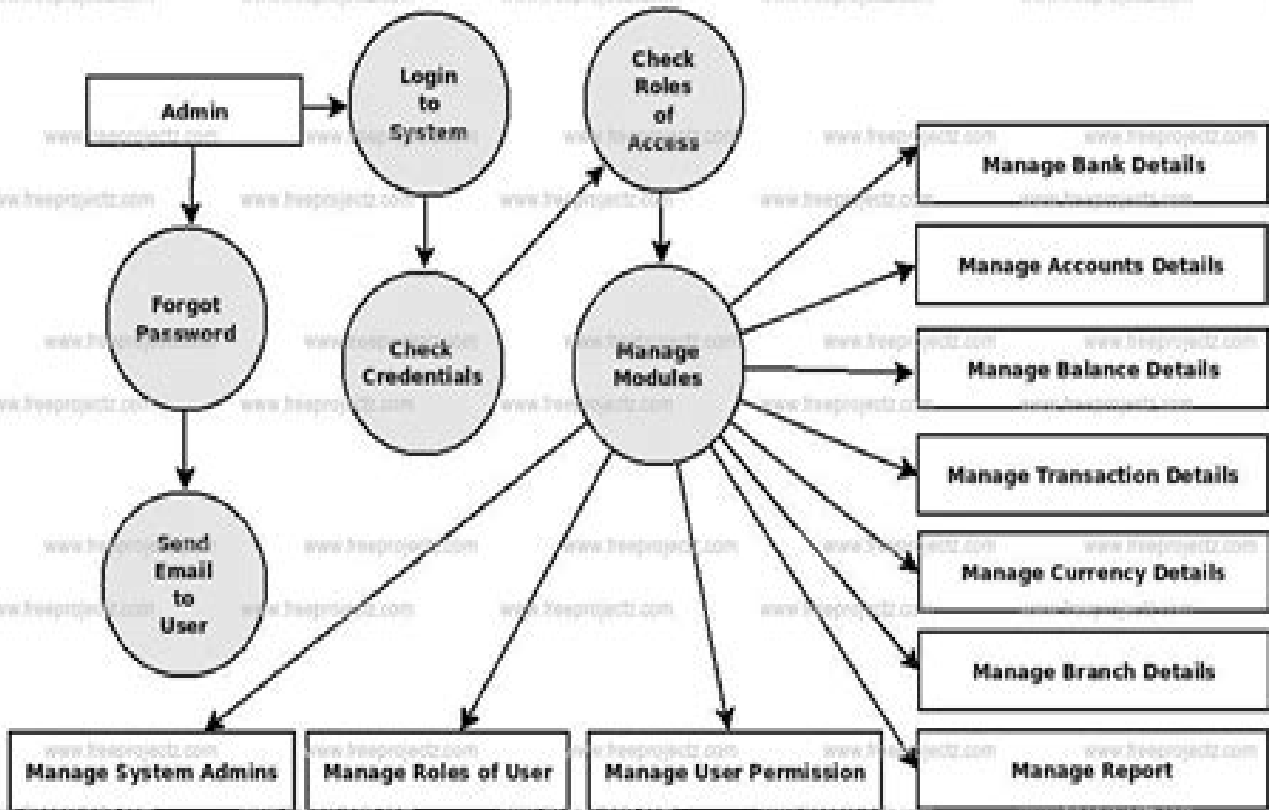
Second Level DFD - Online Banking System
