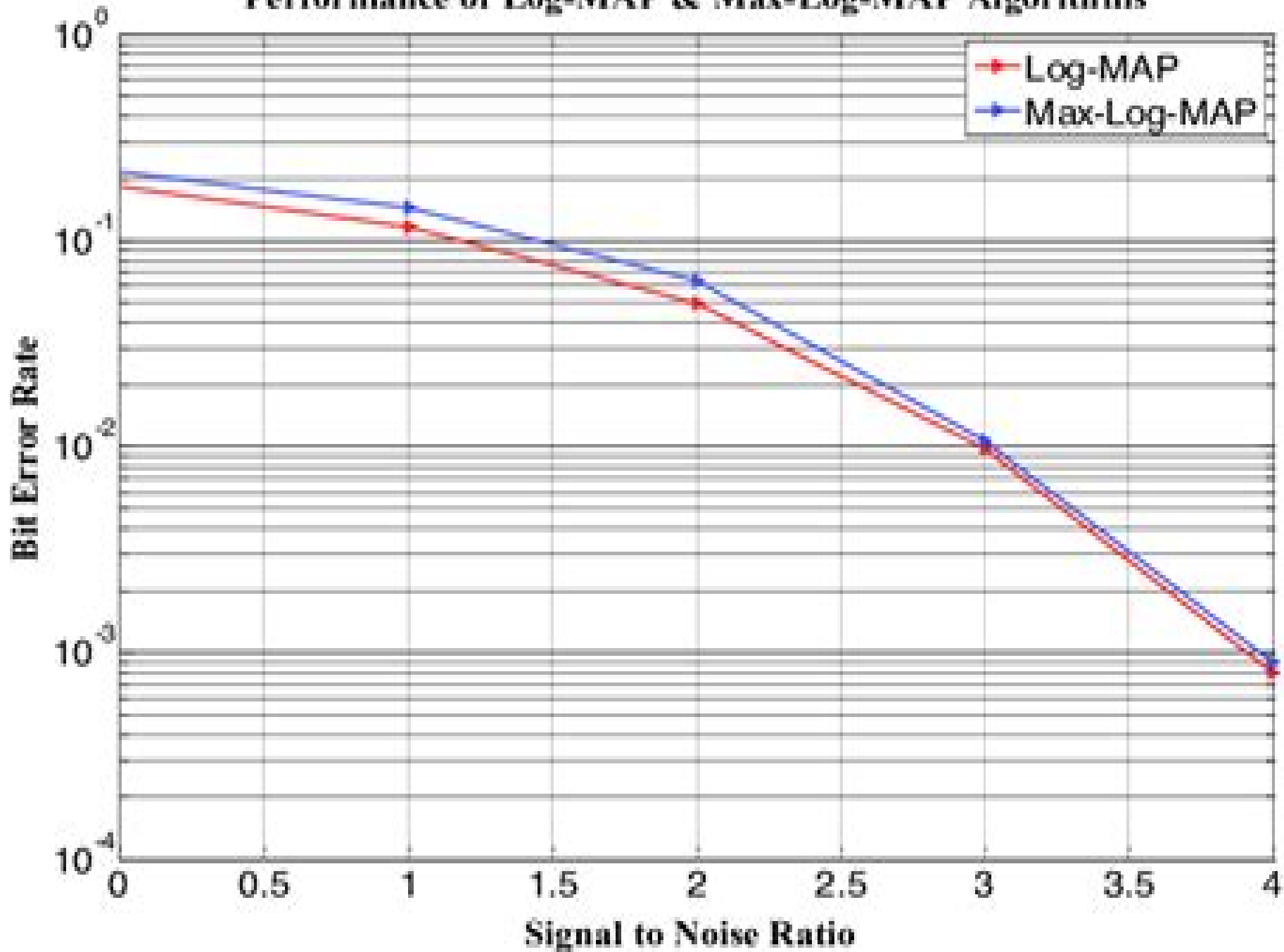
Performance of Log-MAP & Max-Log-MAP Algorithms
