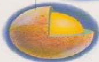
STRUCTURE OF PLUTO
