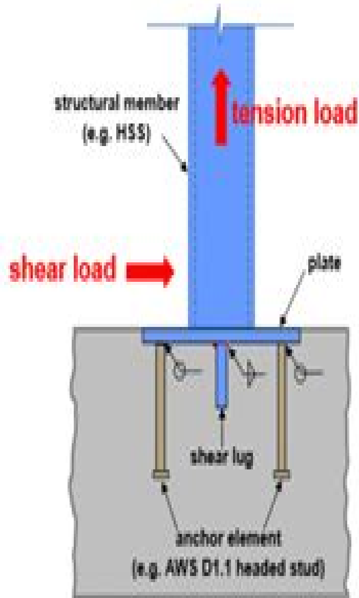
(a) cast-in-place shear lug
