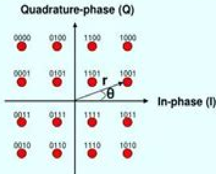
Constellation map for 16 ( =2^4 ) QAM
