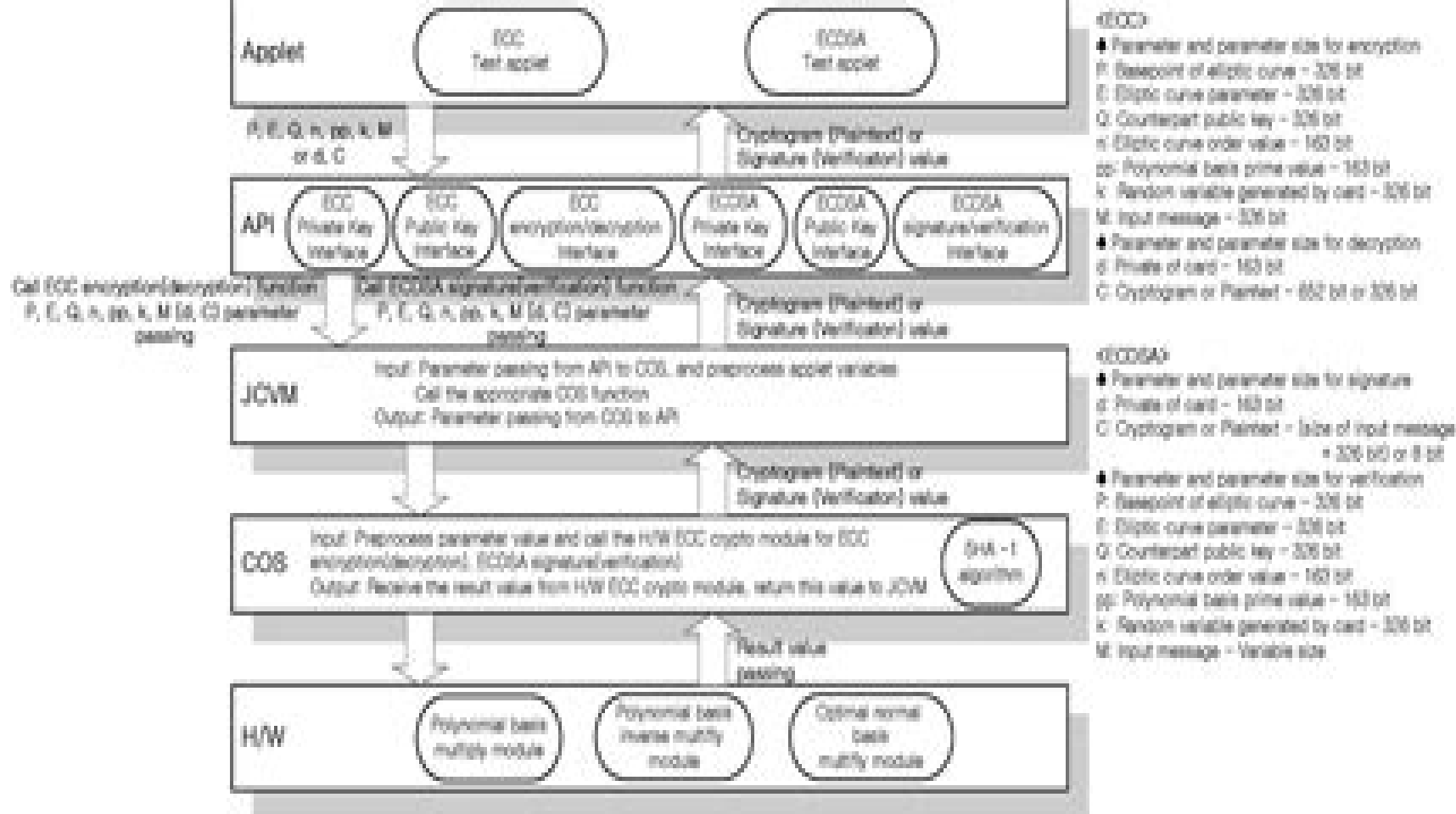
Figure 3. ECC and ECDSA interface
