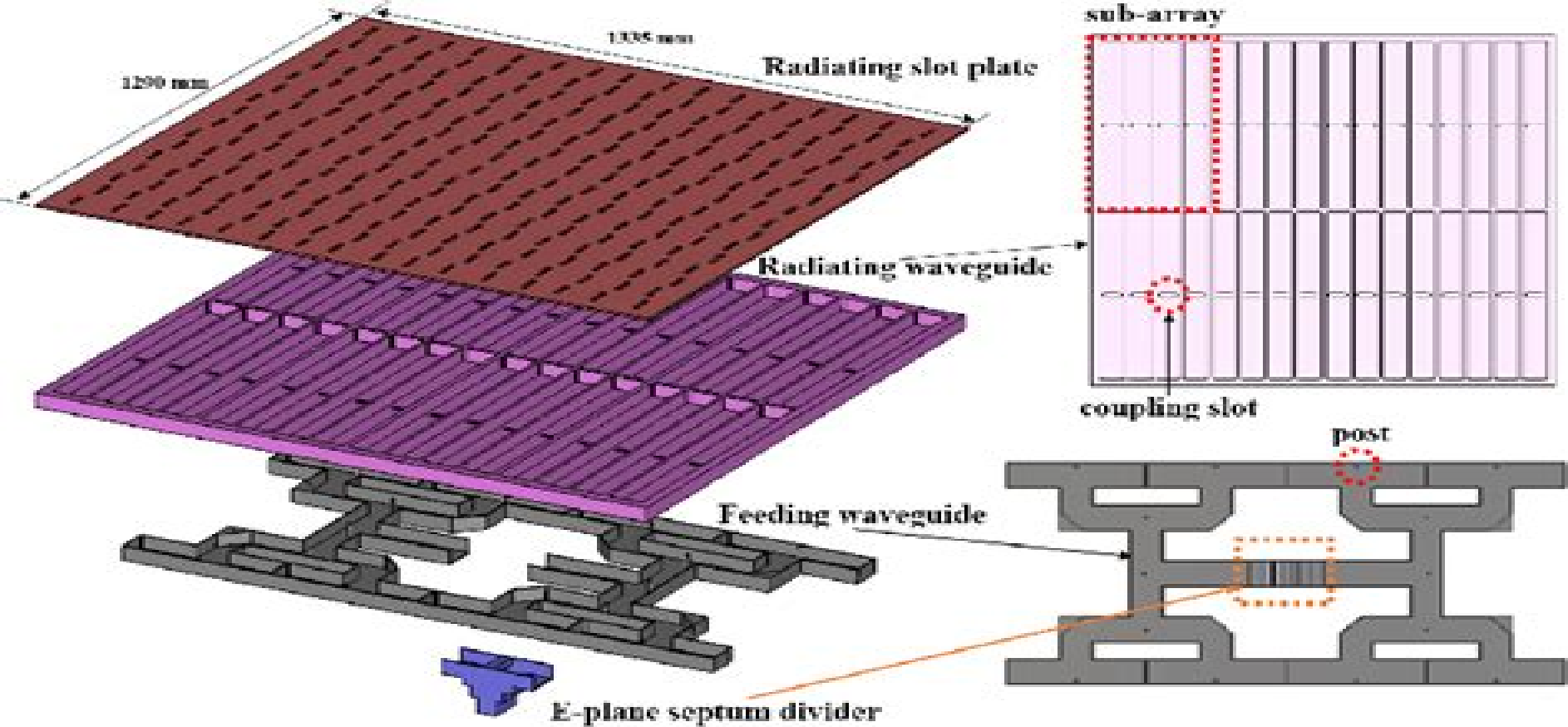
Fig. 1. Designed 16×16 slotted waveguide array antenna structures
