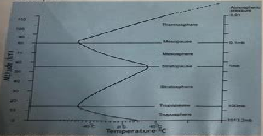
Fig 1.0 The atmosphere: temperature - height diagram
