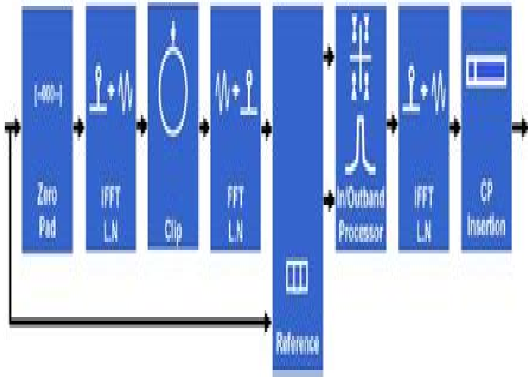
Figure 1. CH Algorithm Block Diagram of the Necessary Processing
