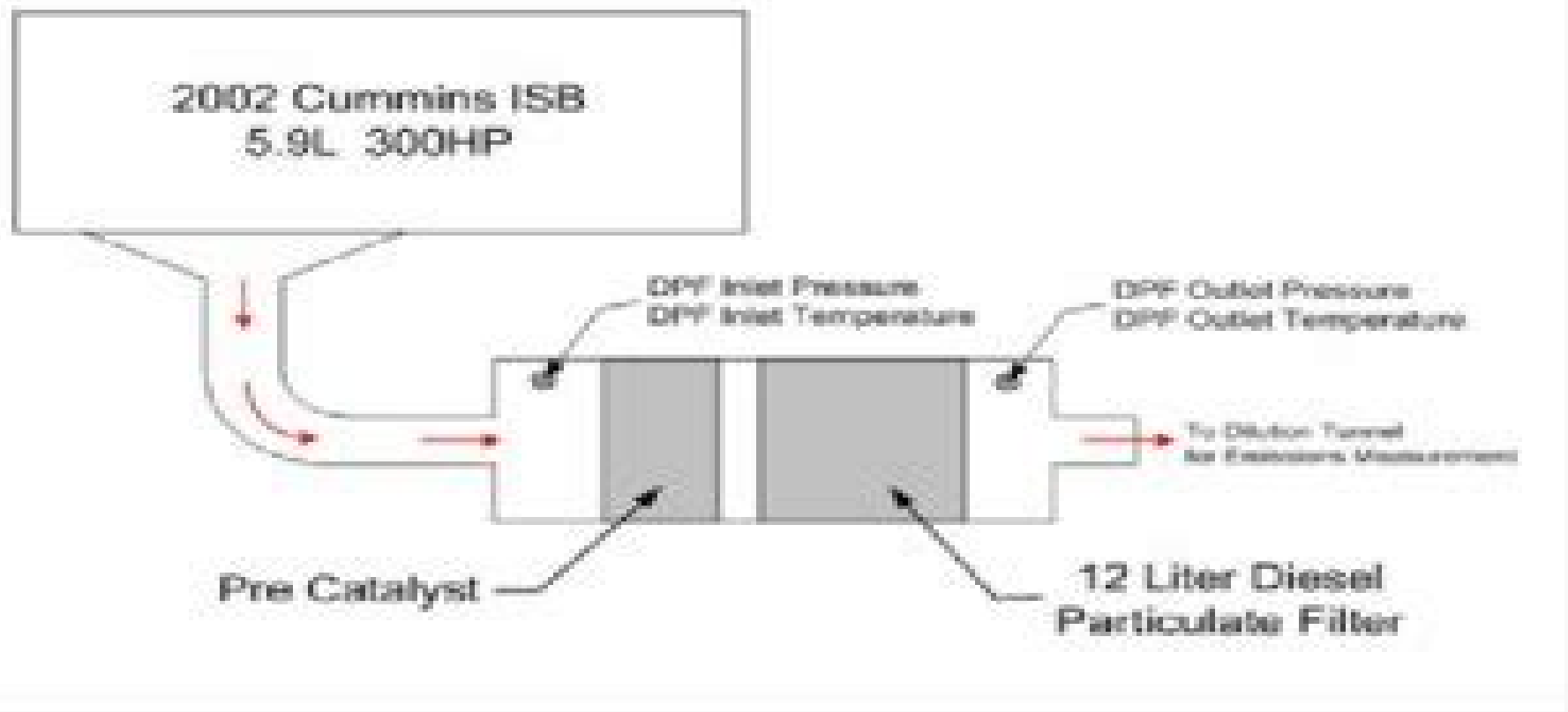
Figure 1. Experimental Setup
