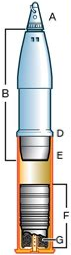
semifixed ammunition
