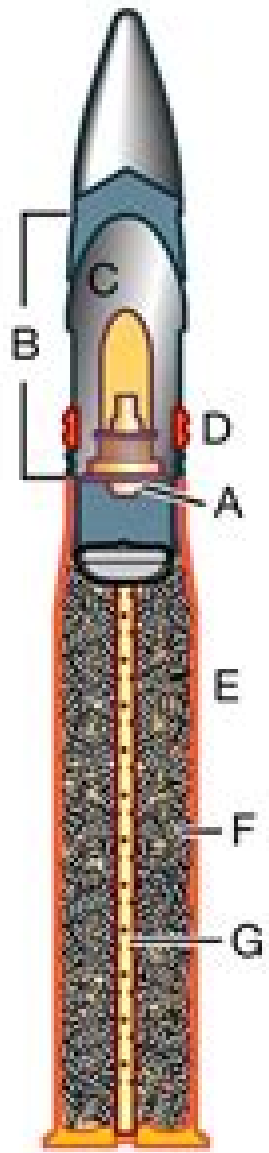
fixed ammunition
