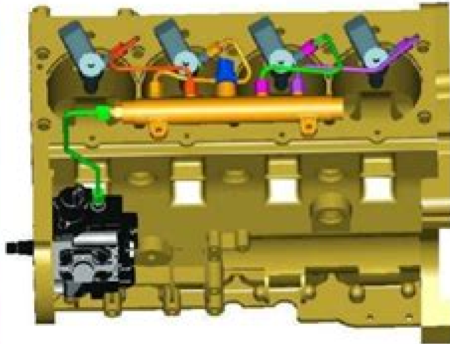
CRDI - COMMON RAIL SYSTEM
