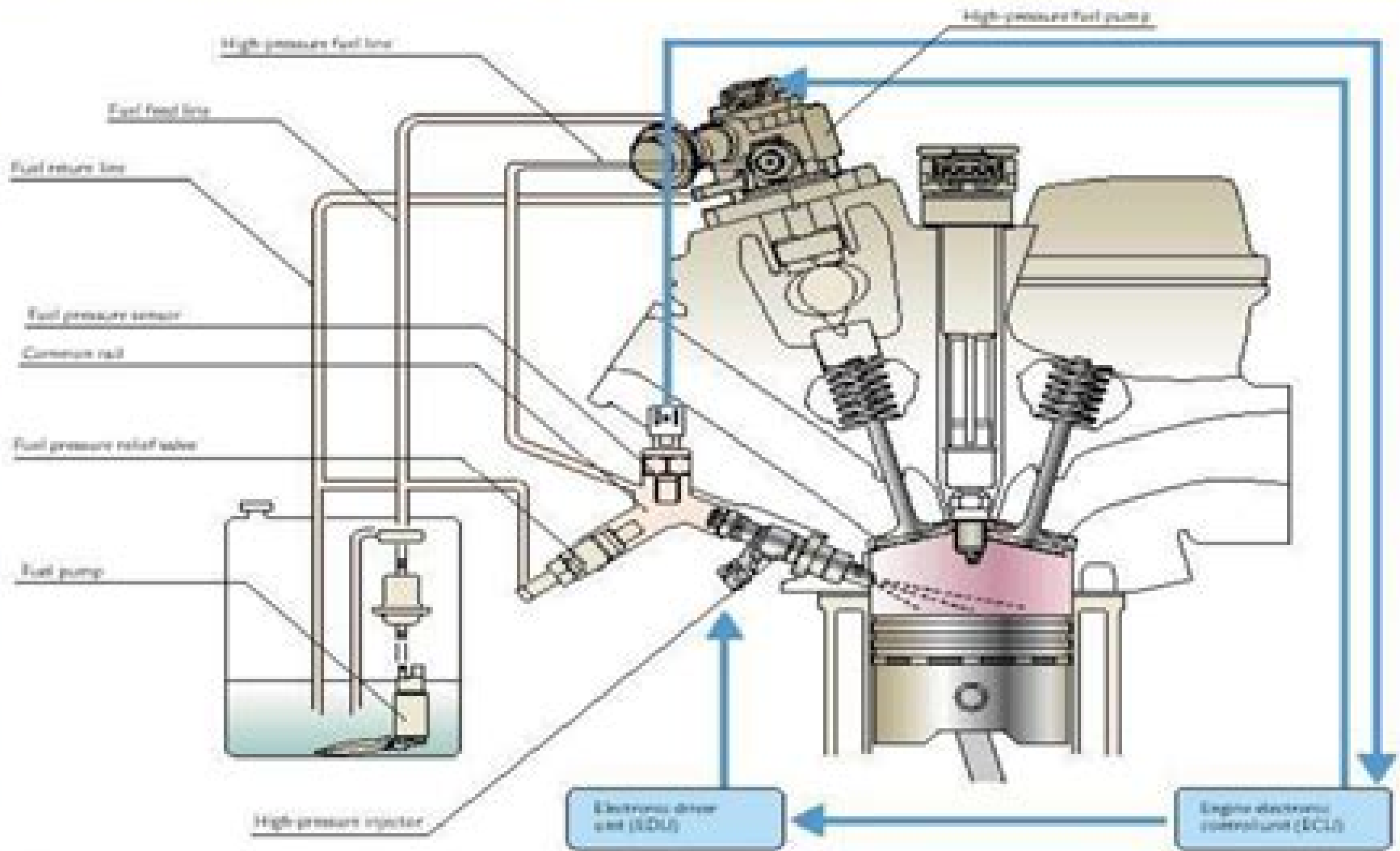
■ Gasoline direct injection system
