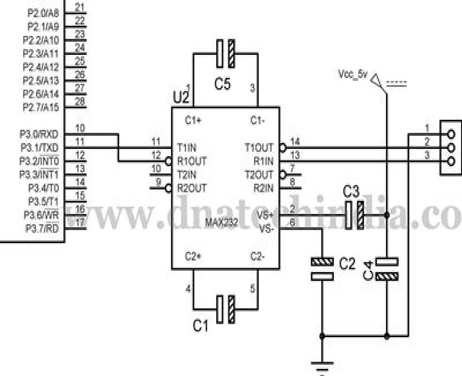
Interfacing Barcode Scanner to Microcontroller
