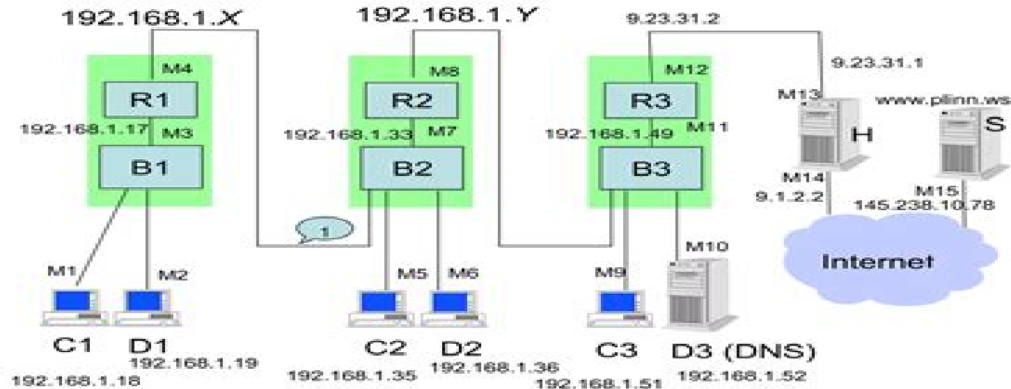
Figure 1: A small corporate network (exercise 2.3).
