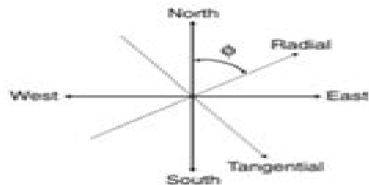
Figure 1. Seismograms are generally recorded with a vertical (not shown) and north and east components. Analysis is often easier when these observations are rotated into the radial-tangential coordinates, where P-SV-Rayleigh waves are separated from SH-Love waves. Formally the radial is the direction along the great circle connecting the epicenter and seismometer and is positive in a direction away from the source.
