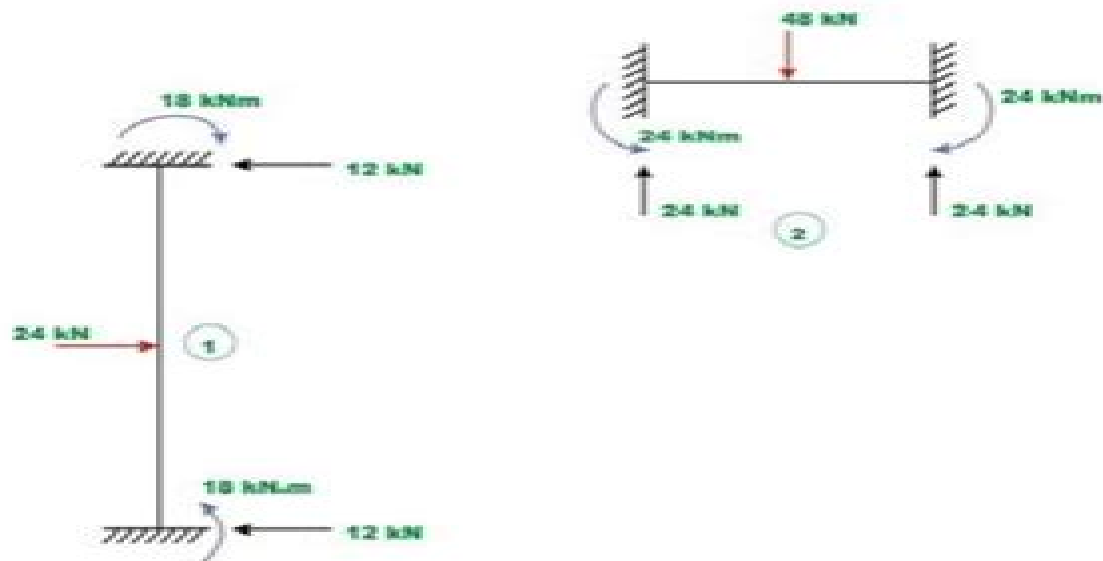
Fig 2.14 Fixed end action due to external loading in element 1 and 2
