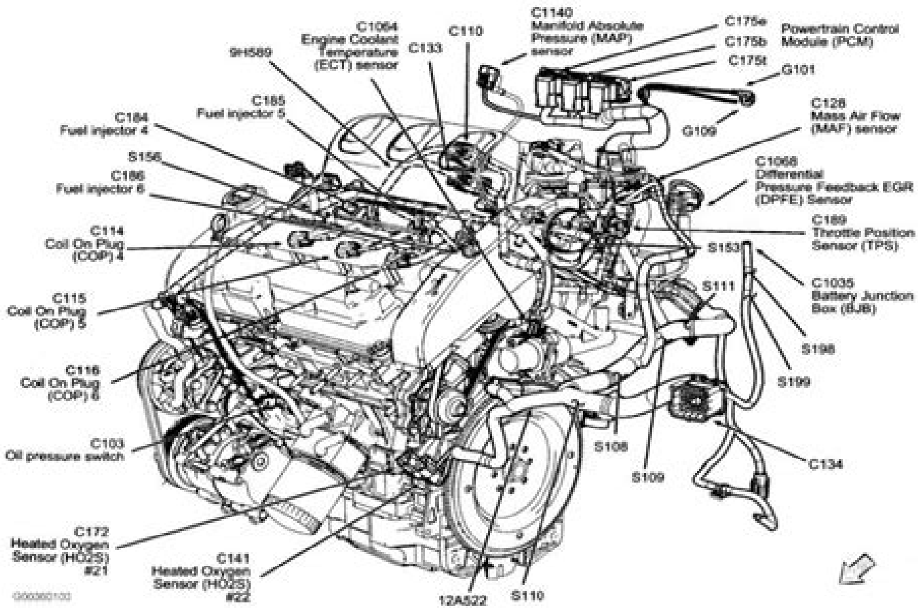
Fig 2: Left Rear Of Engine (3.0L)
