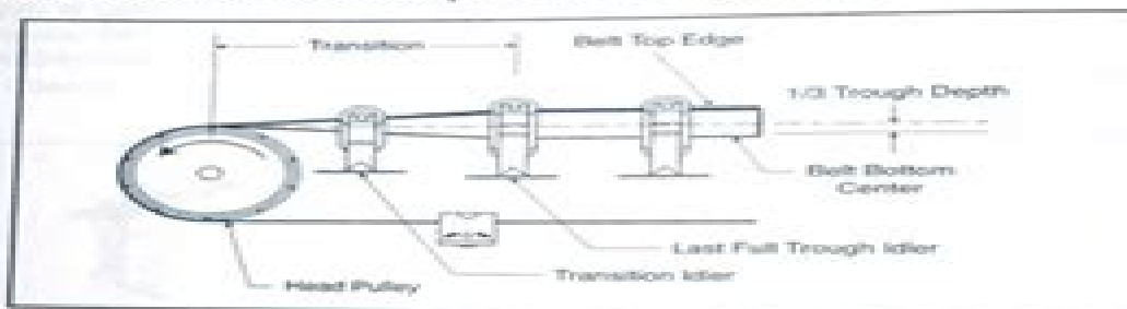
Figure 7.26 One third trough transition from last fully troughed idler to pulley
