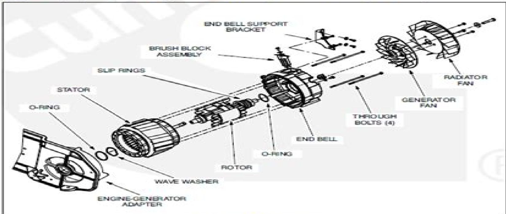
FIGURE 6-1. GENERATOR
