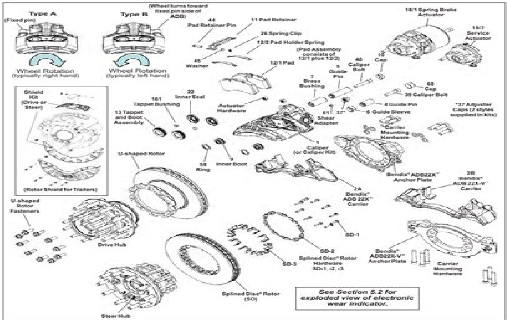
FIGURE 8 - EXPLODED VIEW - BENDIX® ADB22X™ AND ADB22X-V™ AIR DISC BRAKES
