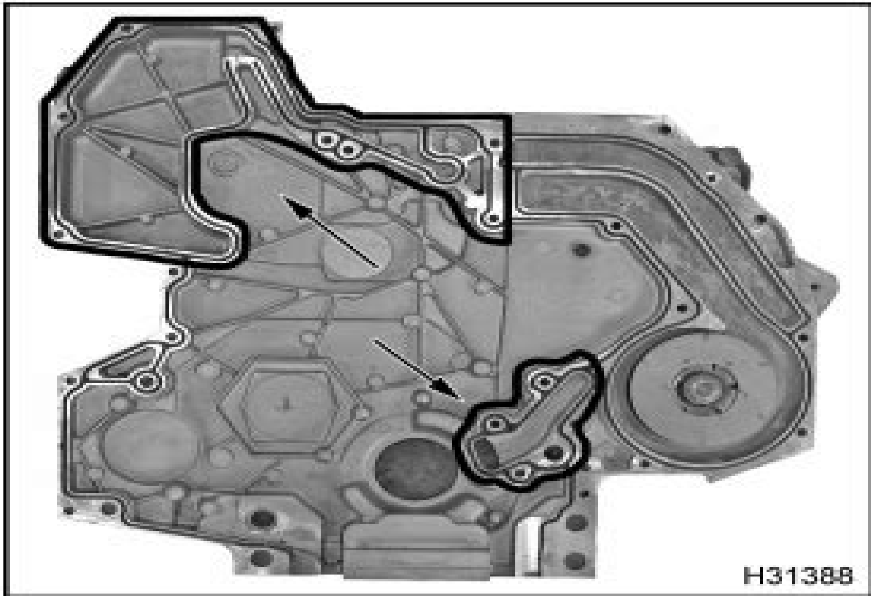
Figure 158 Front cover oil pressure leak locations
