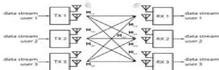
Figure 1: Scheme of the (2 \times 2, 1)^3 interference network.
